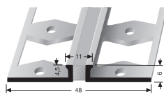
302 S DEHNFUGENPROFIL EXPANSION JOINT PROFILE
