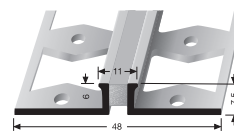
307 S DEHNFUGENPROFIL EXPANSION JOINT PROFILE
