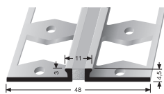
301 S DEHNFUGENPROFIL EXPANSION JOINT PROFILE
