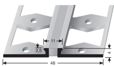
300 S DEHNFUGENPROFIL EXPANSION JOINT PROFILE
