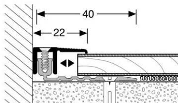
End profile 287
