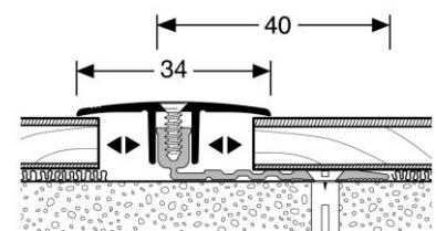
Transition profile 289 with plain surface
