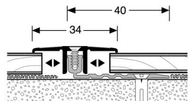
Transition profile 288
