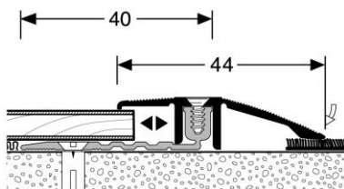
Adaption profile 286
