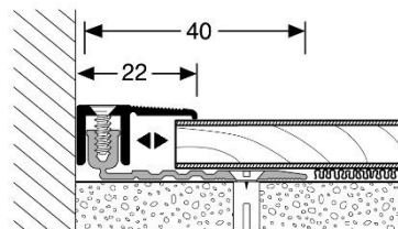
End profile 487
