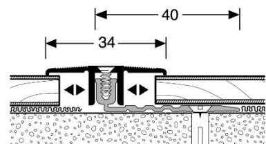
Transition profile 488
