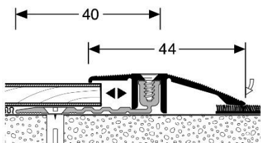
Adaption profile 486
