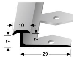
Profil 297 EB
